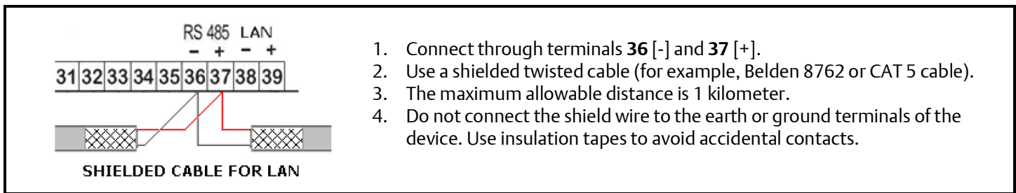
Figure 5-7 - Connecting the Monitoring System
