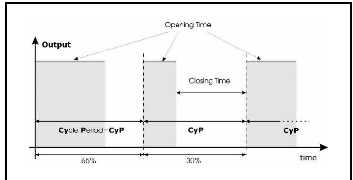
Figure 15-2 - Regulation Diagram
