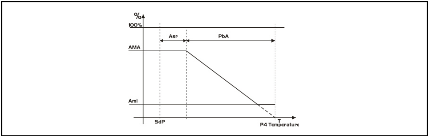
Figure 15-6 - Anti-Sweat Heaters
