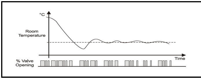
Figure 15-4 - Second Kind Regulation Diagram
